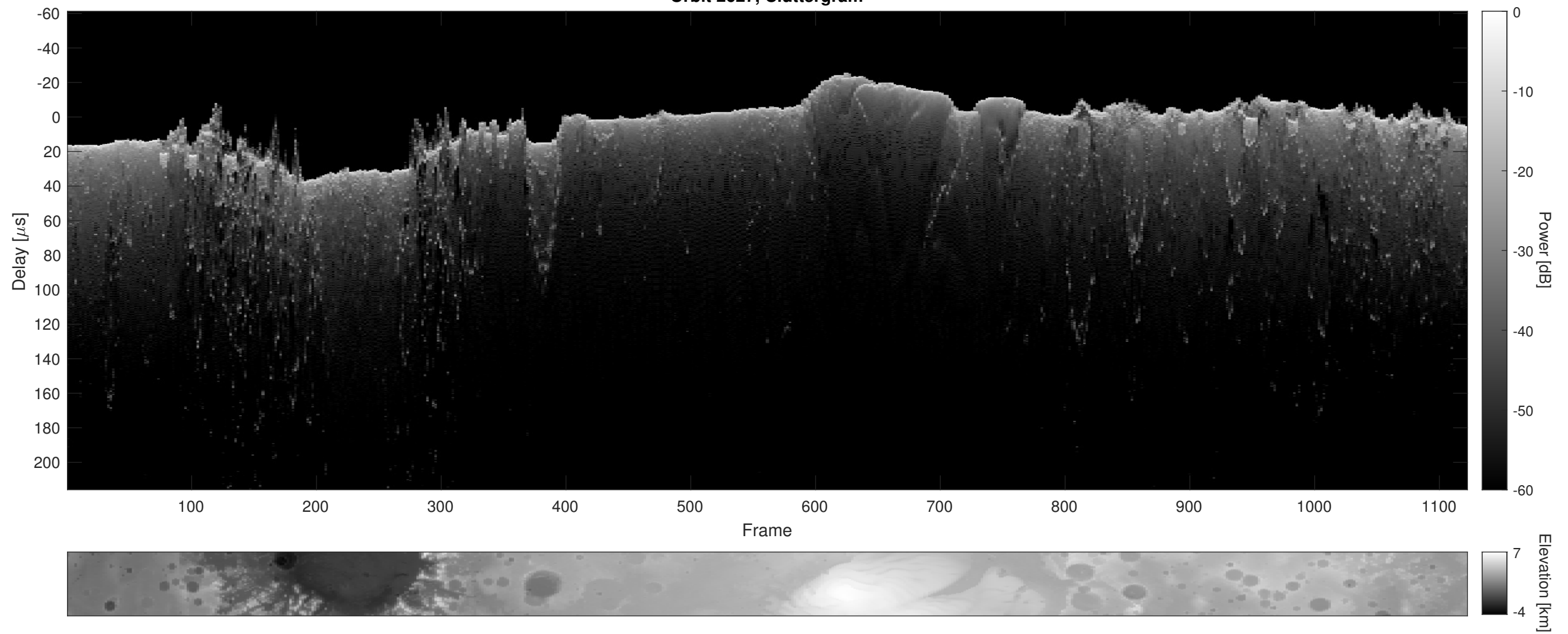
Orbit 2627, Cluttergram
