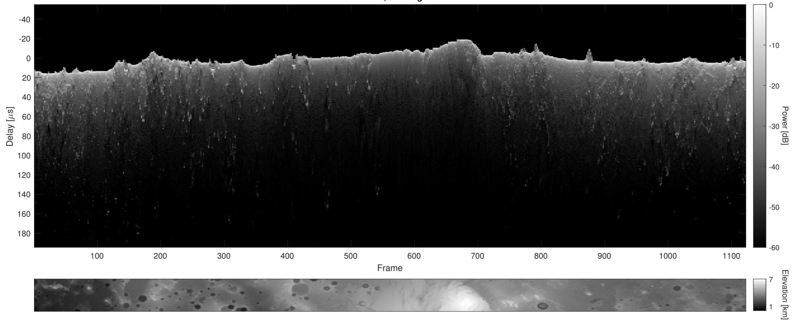
Orbit 2628, Cluttergram
