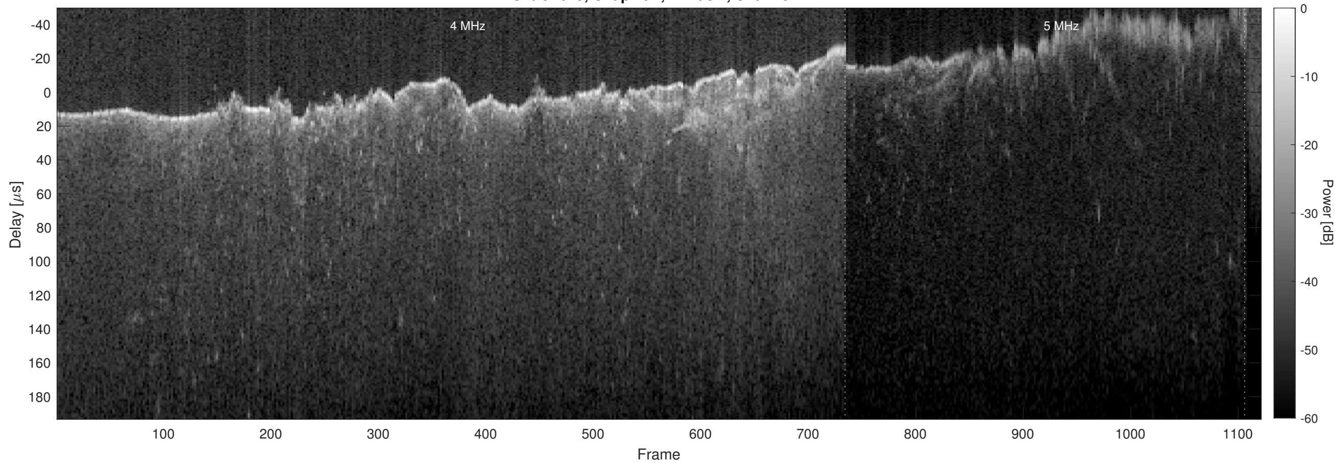
Orbit 2629, Chapman, Window, Channel 2
