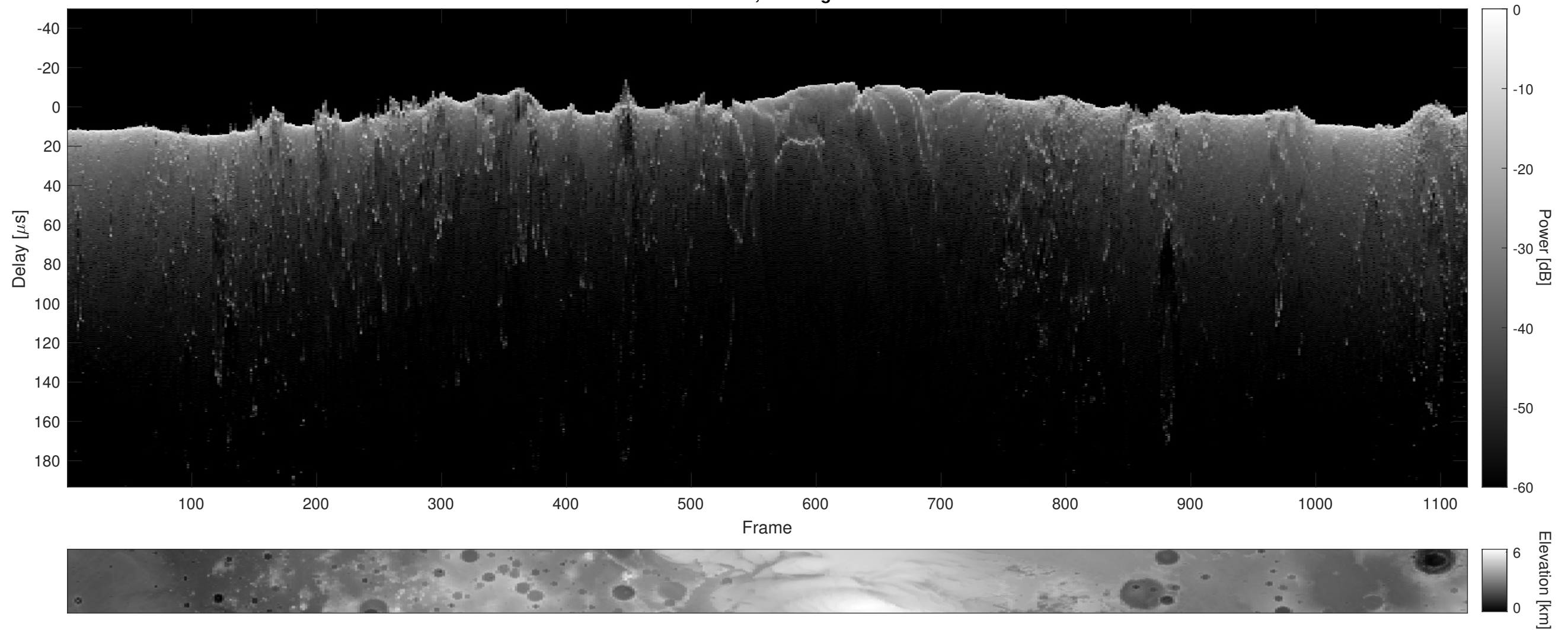
Orbit 2629, Cluttergram
