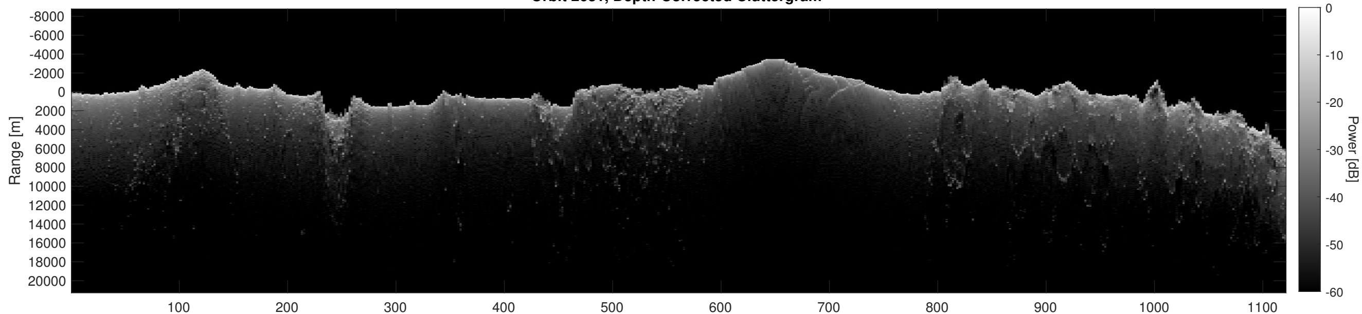
Orbit 2631, Depth-Corrected Cluttergram
