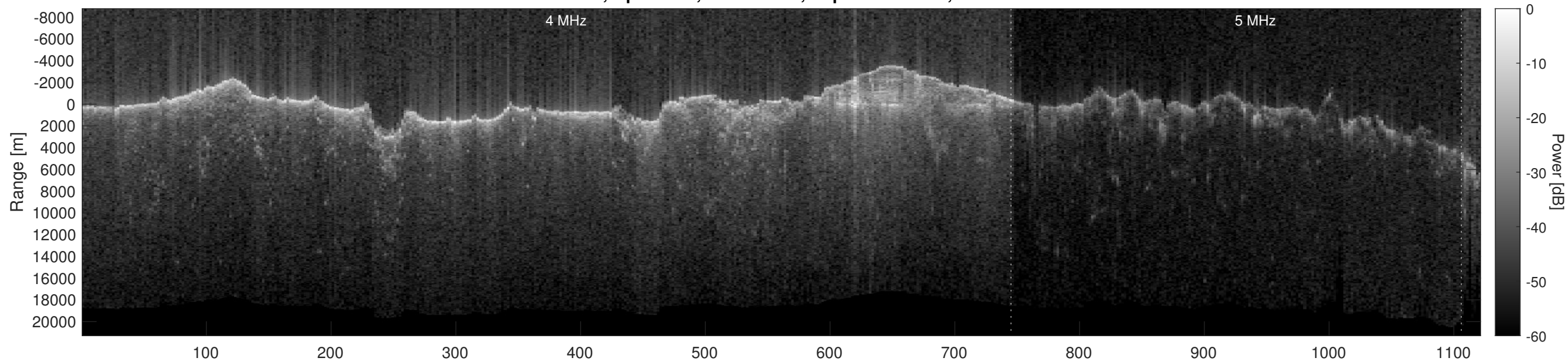
Orbit 2631, Optimized, No Window, Depth-Corrected, Channel 2
