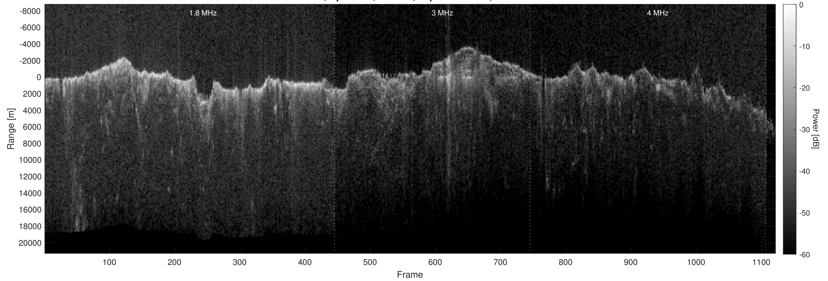
Orbit 2631, Optimized, Window, Depth-Corrected, Channel 2
