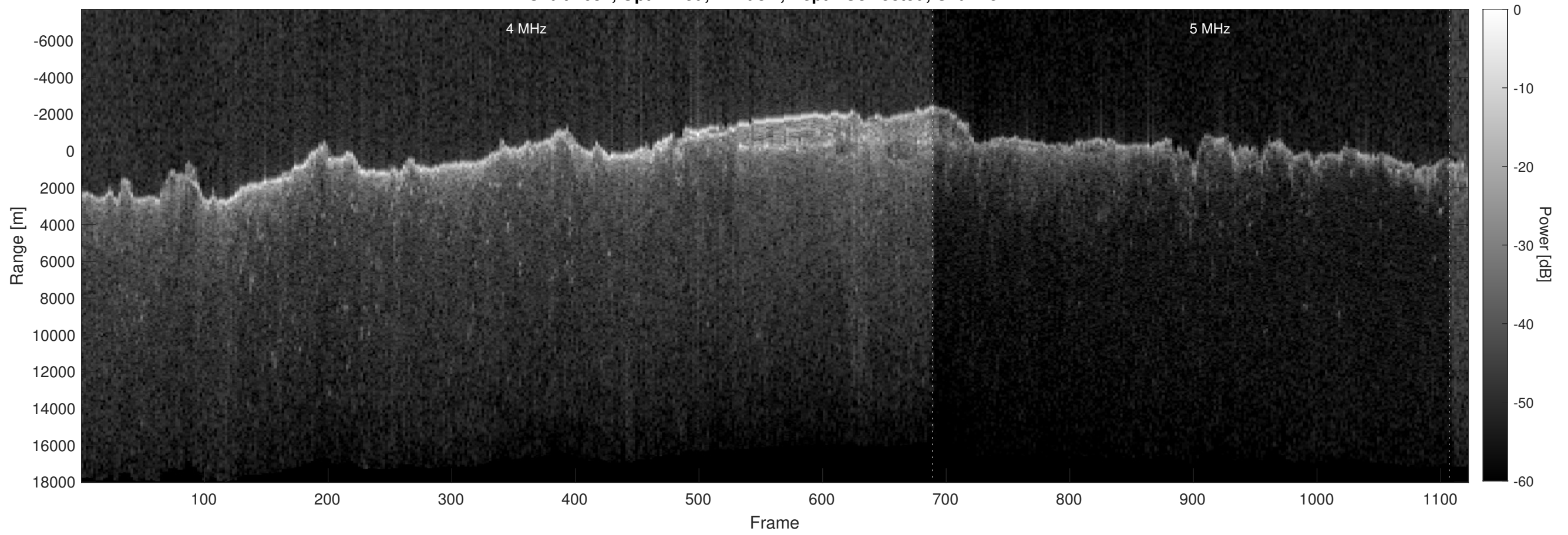
Orbit 2632, Optimized, Window, Depth-Corrected, Channel 2
