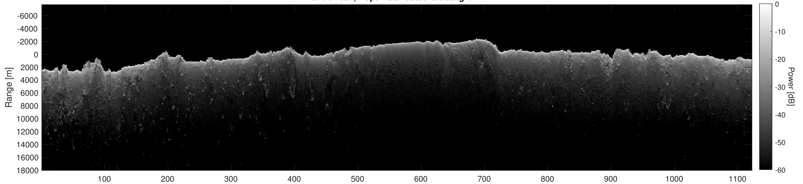
Orbit 2632, Depth-Corrected Cluttergram
