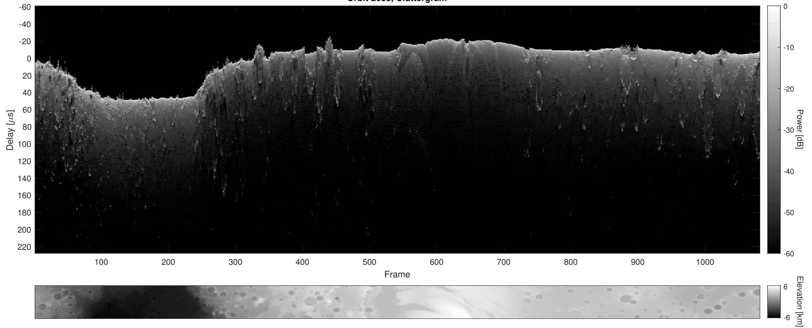
Orbit 2633, Cluttergram
