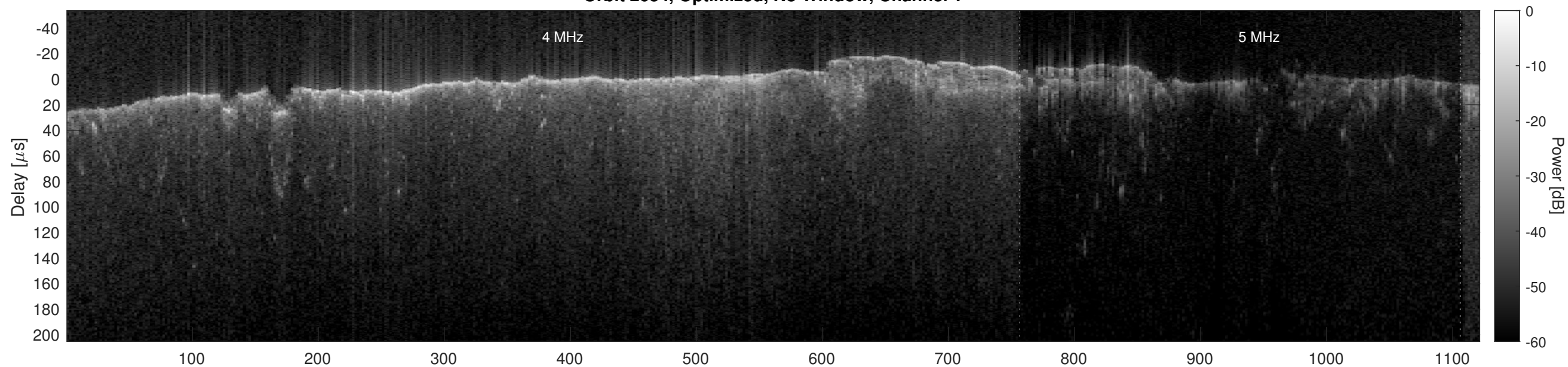
Orbit 2634, Optimized, No Window, Channel 2
