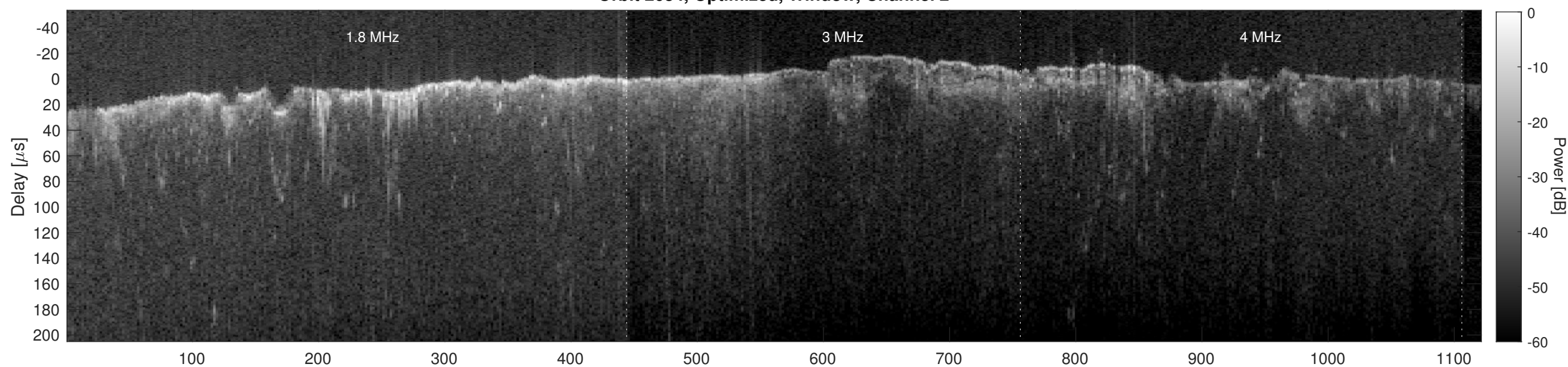
Orbit 2634, Cluttergram
