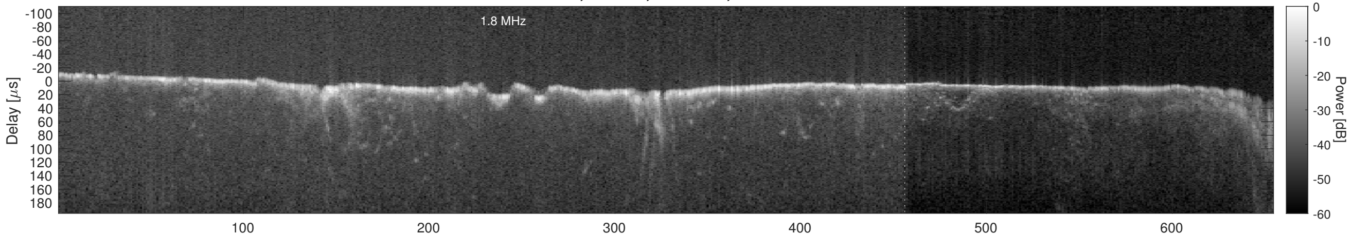
Orbit 2635, Window, Channel 2, Chapman
