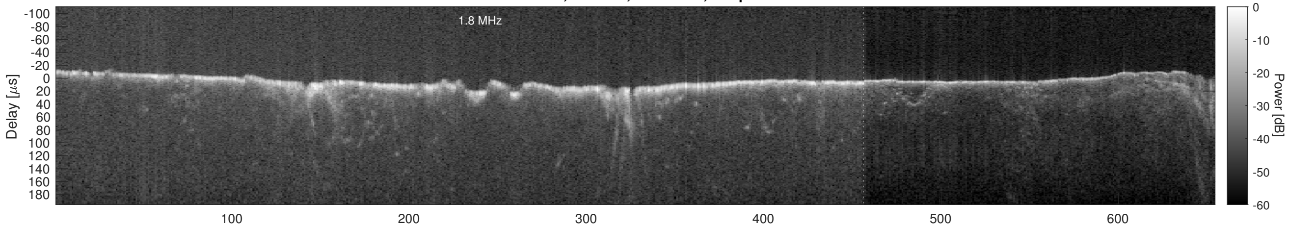
Orbit 2635, Window, Channel 2, Optimized
