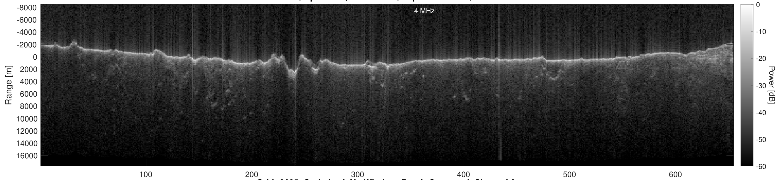
Orbit 2635, Optimized, No Window, Depth-Corrected, Channel 2
