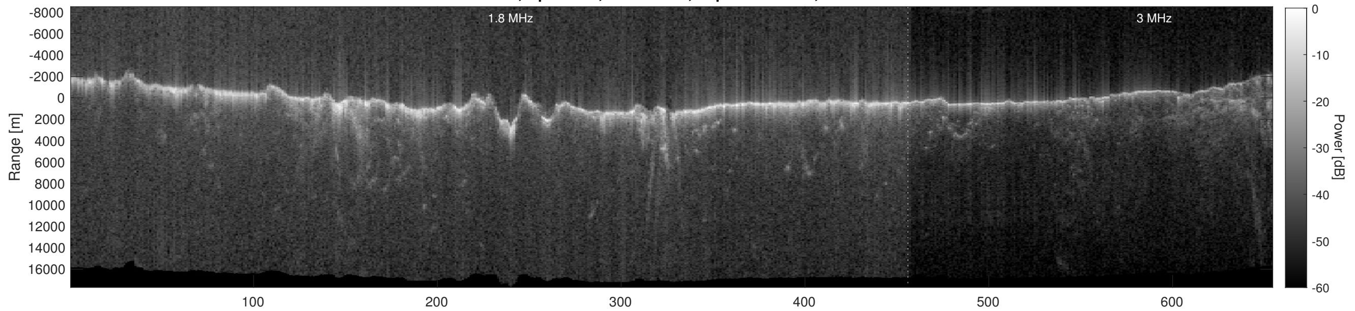
Orbit 2635, Depth-Corrected Cluttergram
