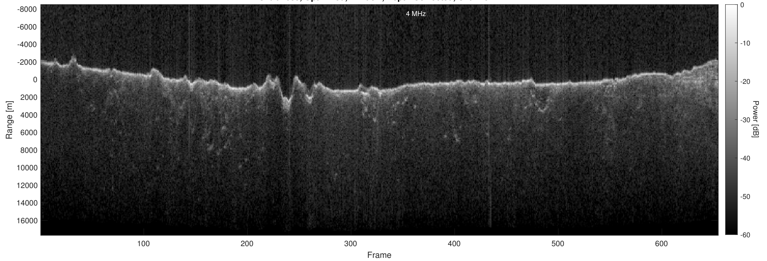
Orbit 2635, Optimized, Window, Depth-Corrected, Channel 2
