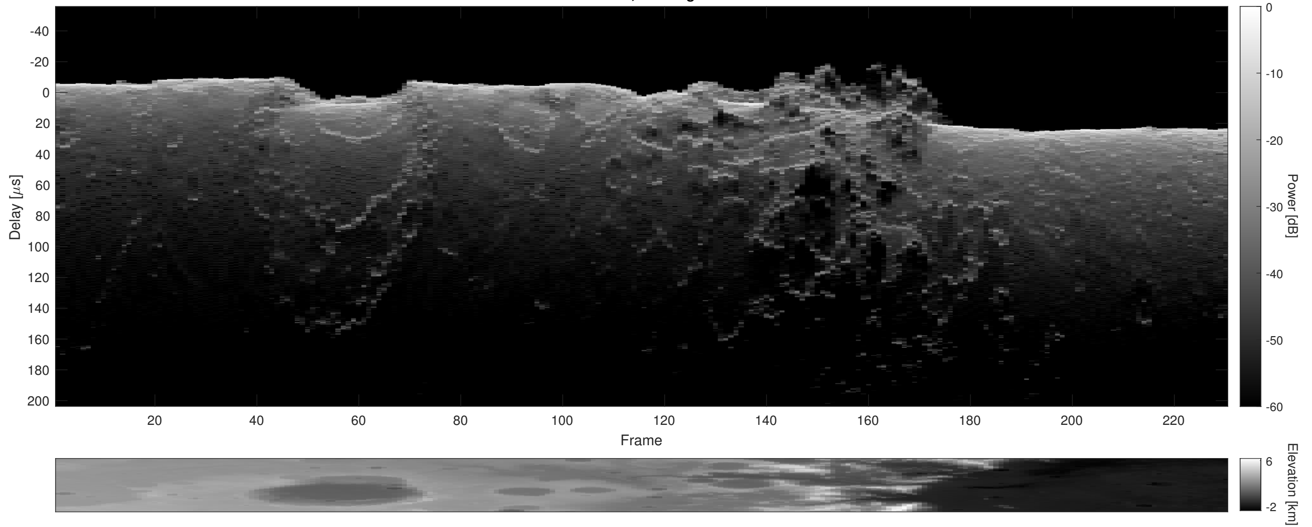
Orbit 2636, Cluttergram
