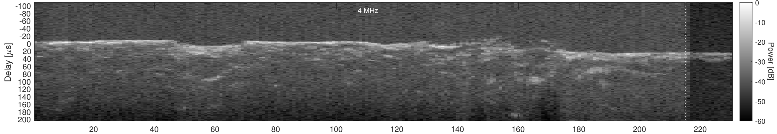
Orbit 2636, Cluttergram
