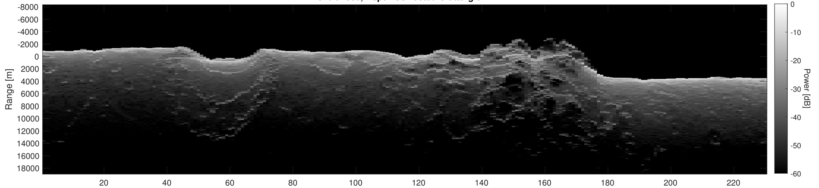
Orbit 2636, Depth-Corrected Cluttergram
