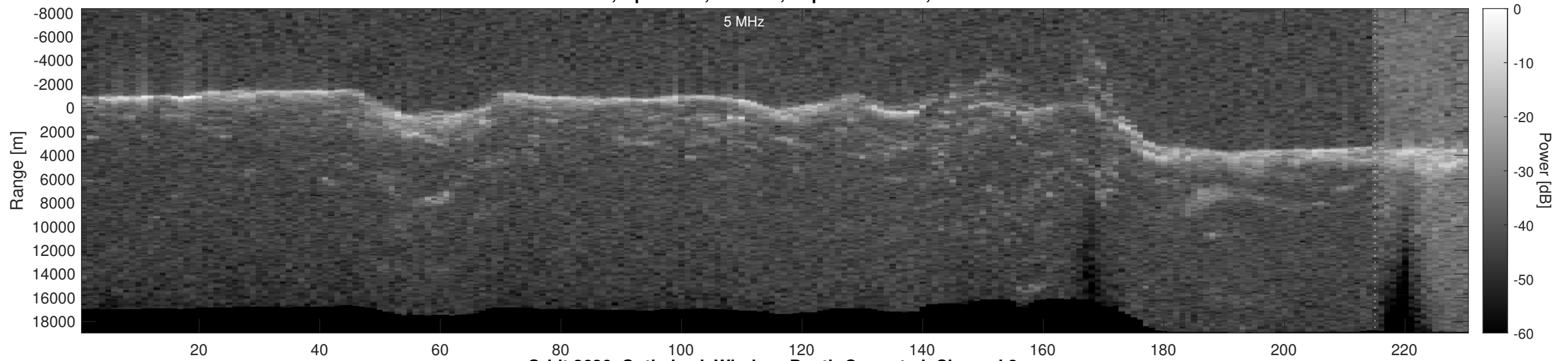
Orbit 2636, Optimized, Window, Depth-Corrected, Channel 2
