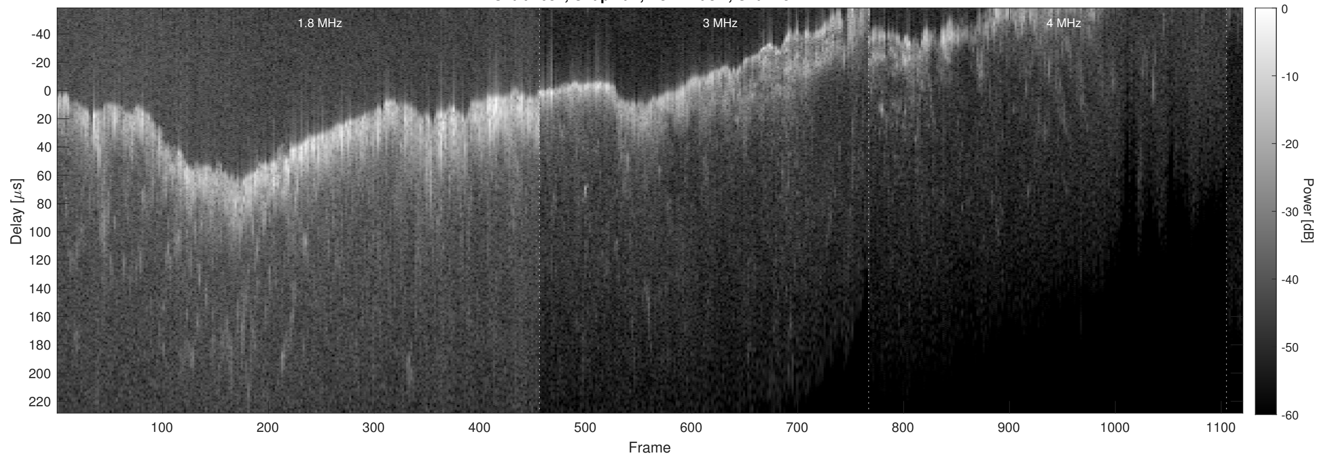
Orbit 2637, Chapman, No Window, Channel 2
