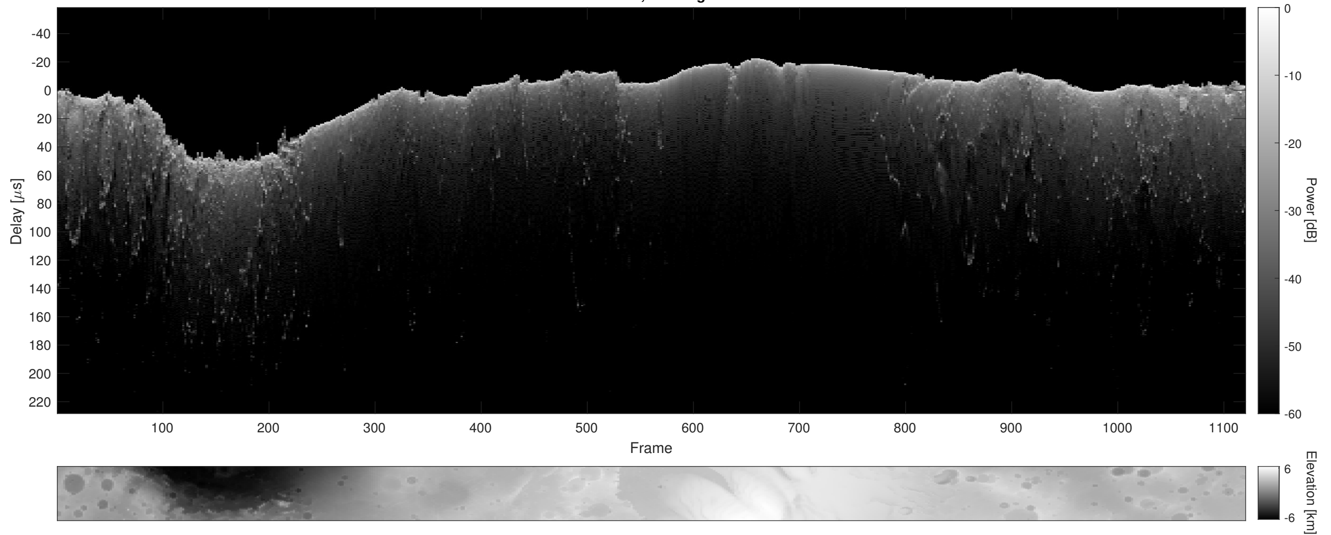
Orbit 2637, Cluttergram
