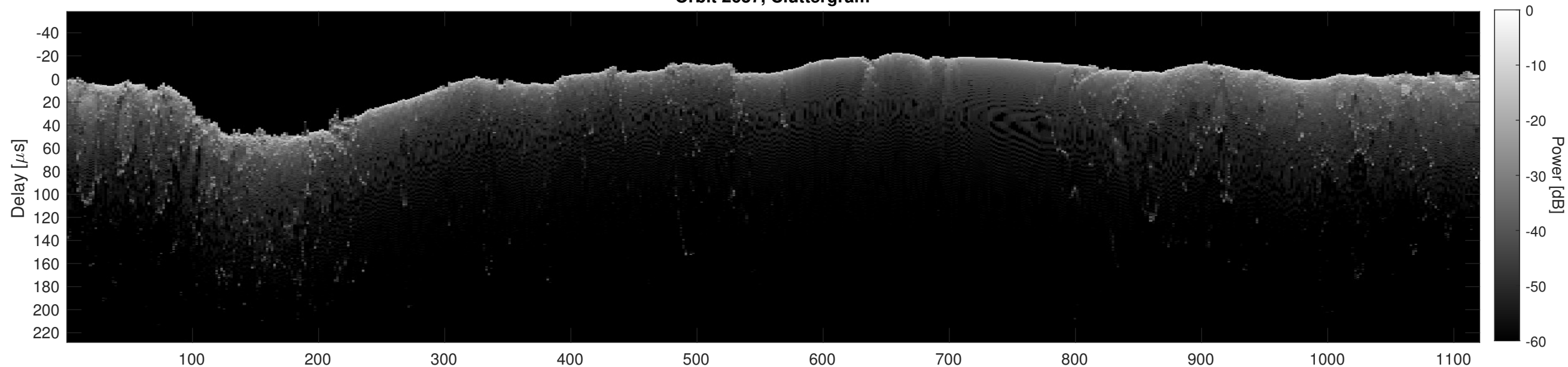
Orbit 2637, Cluttergram
