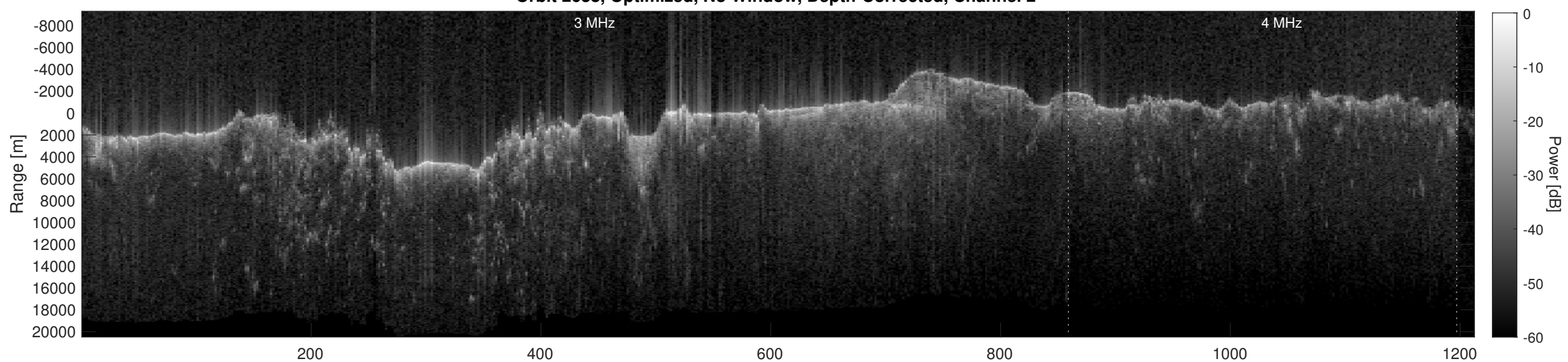
Orbit 2638, Depth-Corrected Cluttergram
