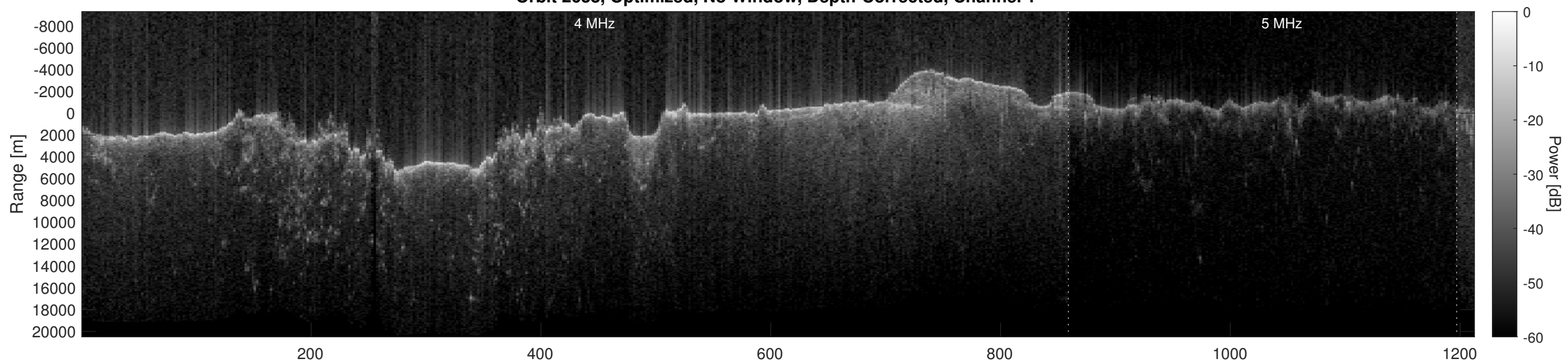
Orbit 2638, Optimized, No Window, Depth-Corrected, Channel 2
