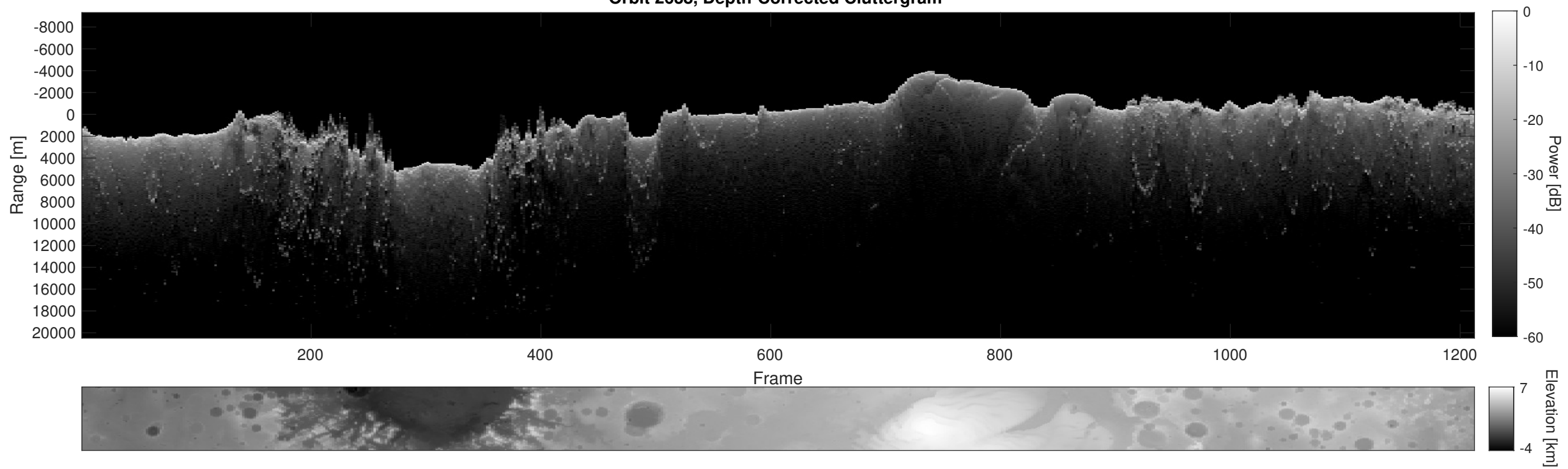
Orbit 2638, Depth-Corrected Cluttergram
