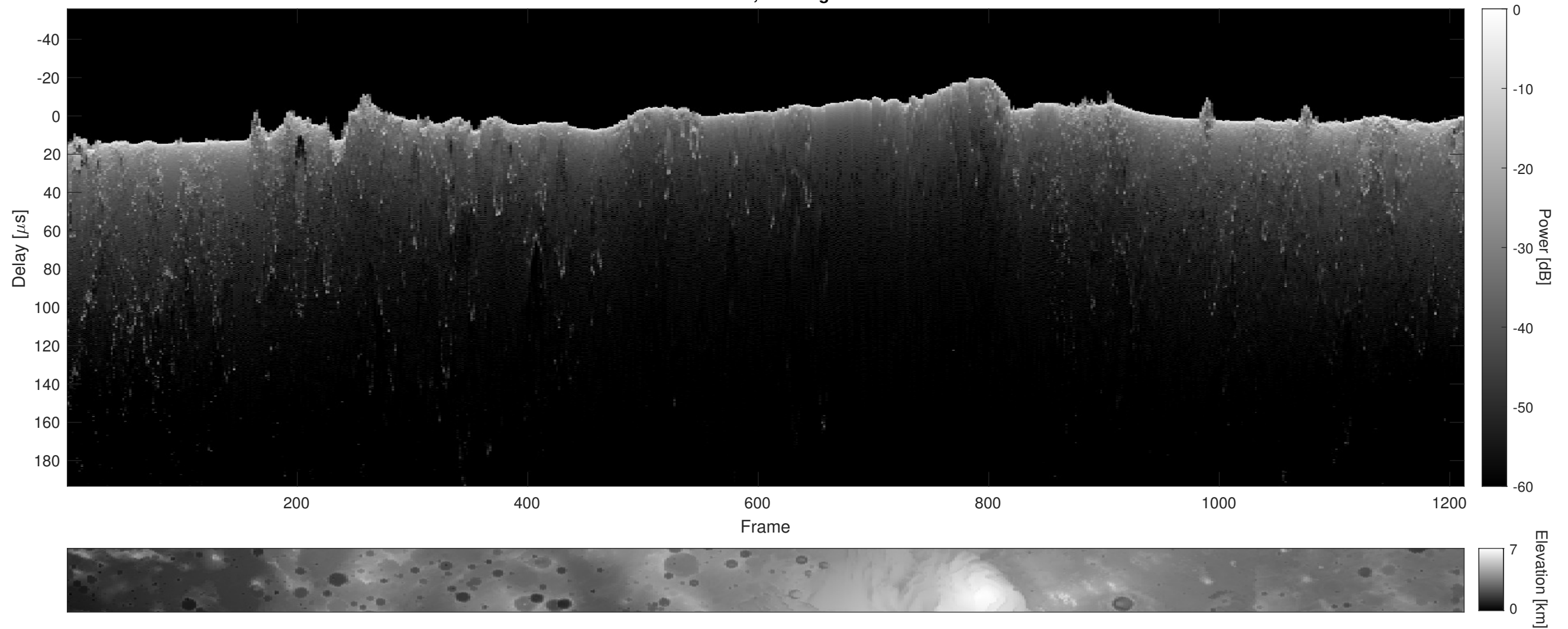
Orbit 2639, Cluttergram
