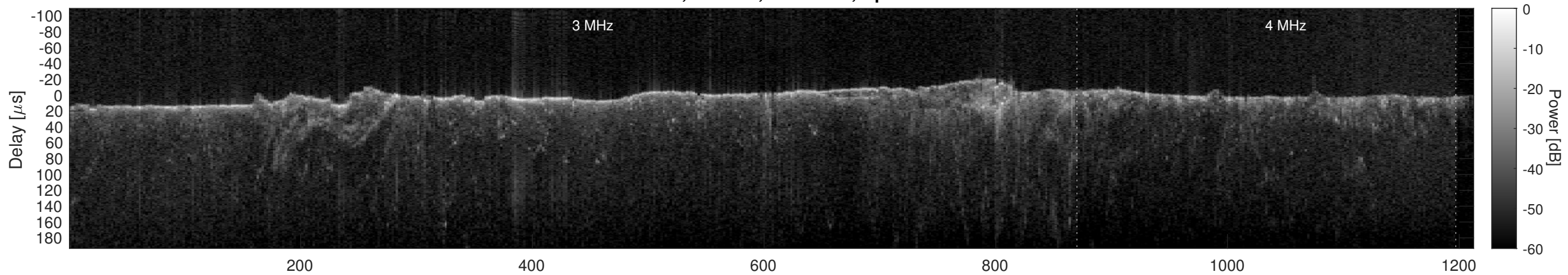
Orbit 2639, Cluttergram
