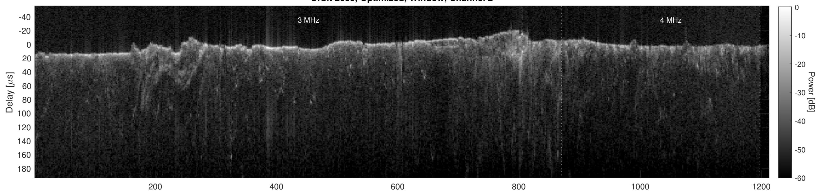
Orbit 2639, Cluttergram
