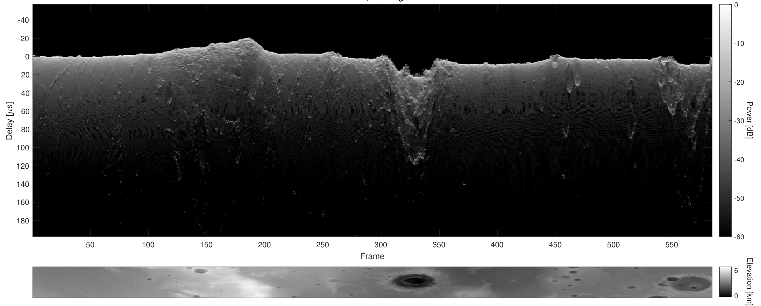
Orbit 2642, Cluttergram
