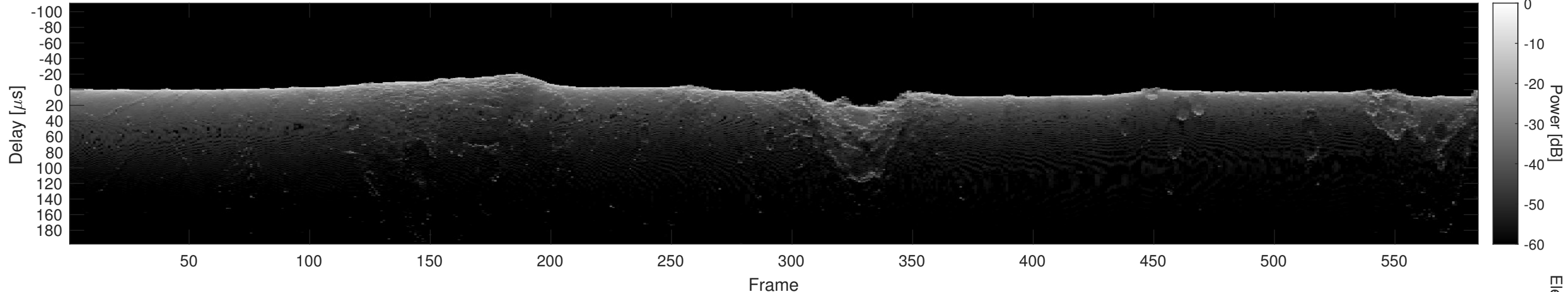
Orbit 2642, Cluttergram
