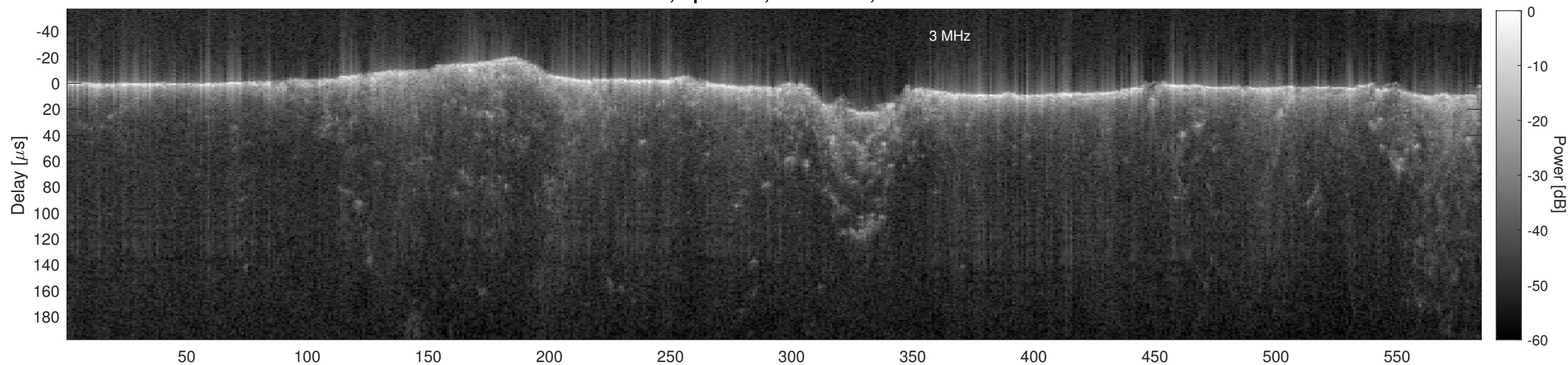
Orbit 2642, Cluttergram
