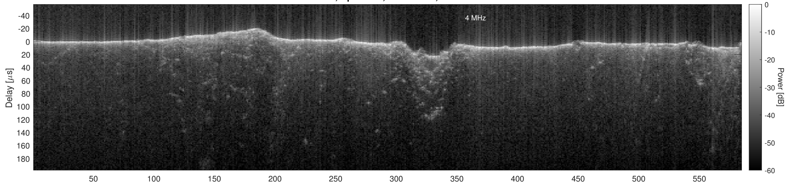
Orbit 2642, Optimized, No Window, Channel 2
