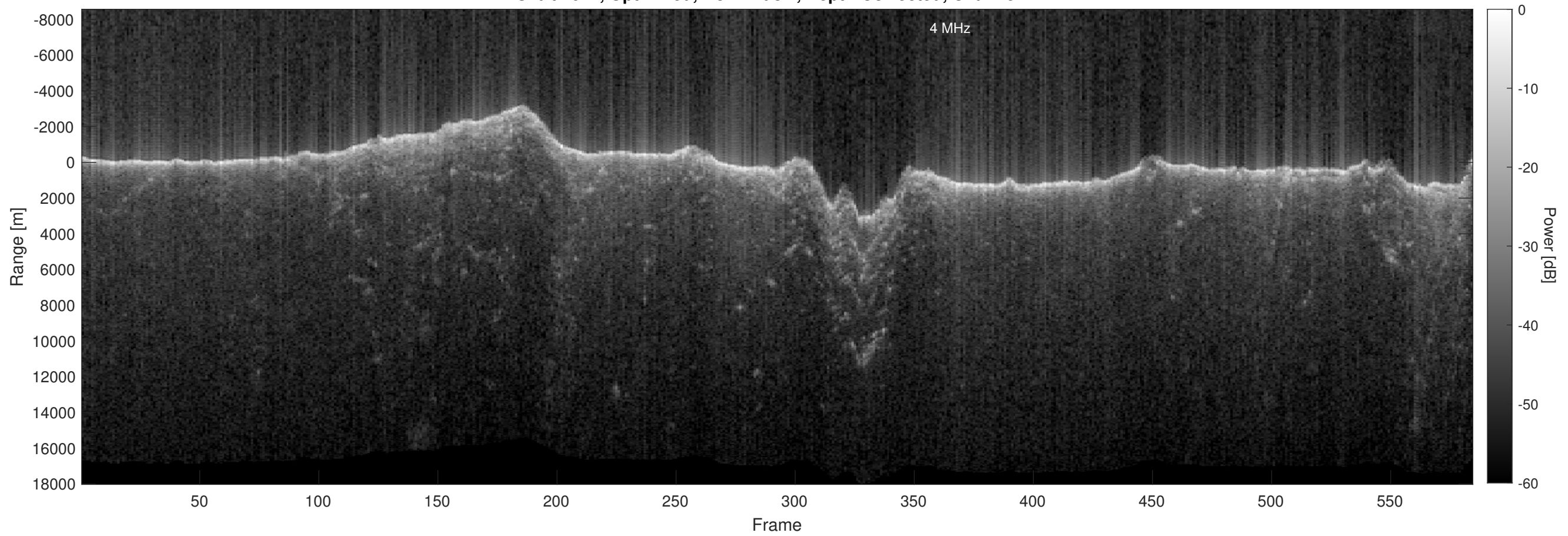
Orbit 2642, Optimized, No Window, Depth-Corrected, Channel 2
