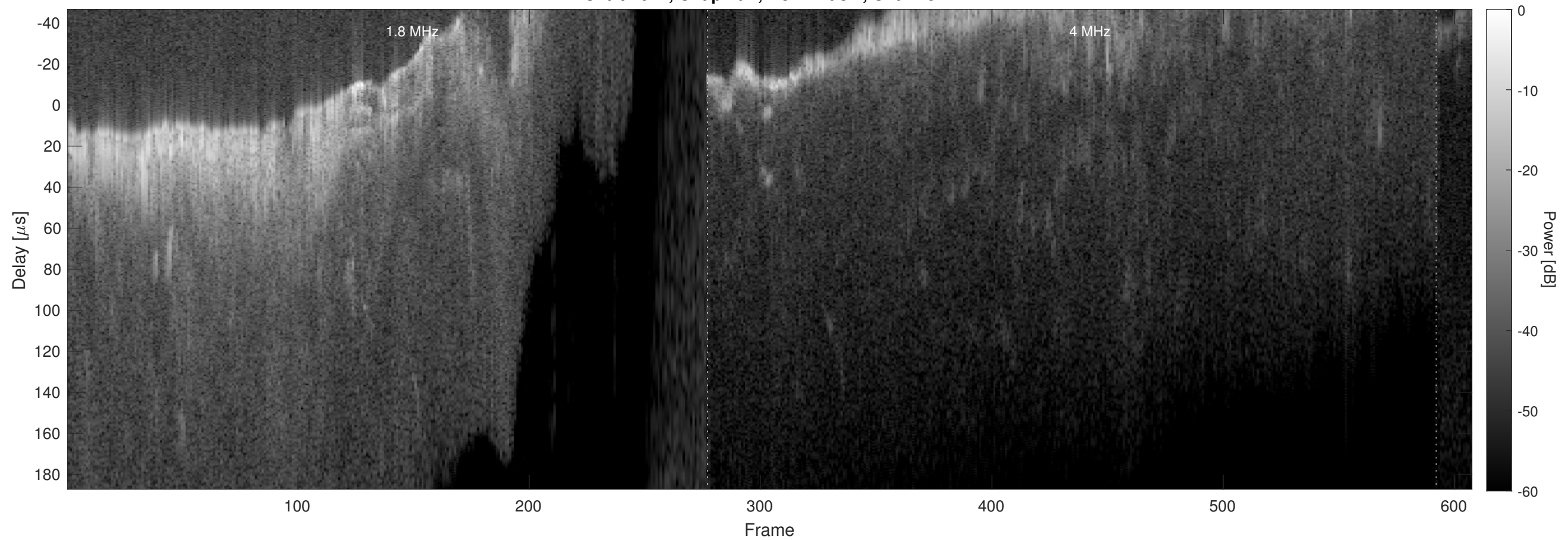
Orbit 2644, Chapman, No Window, Channel 2
