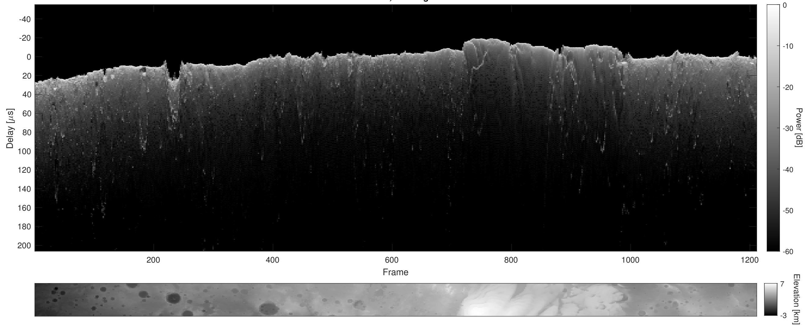
Orbit 2645, Cluttergram
