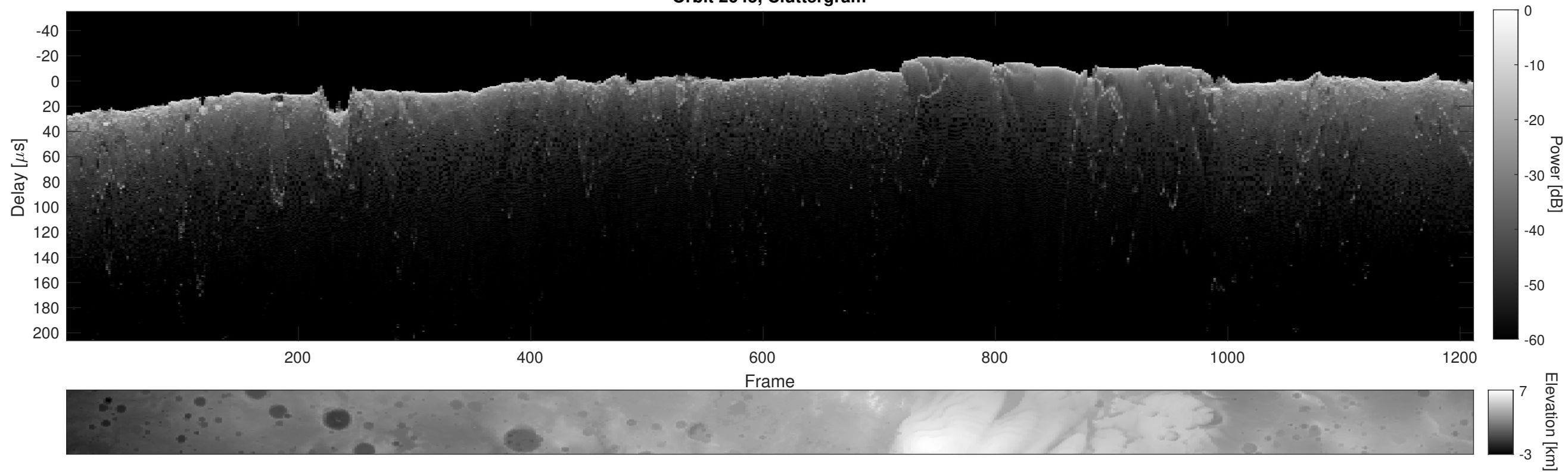
Orbit 2645, Cluttergram
