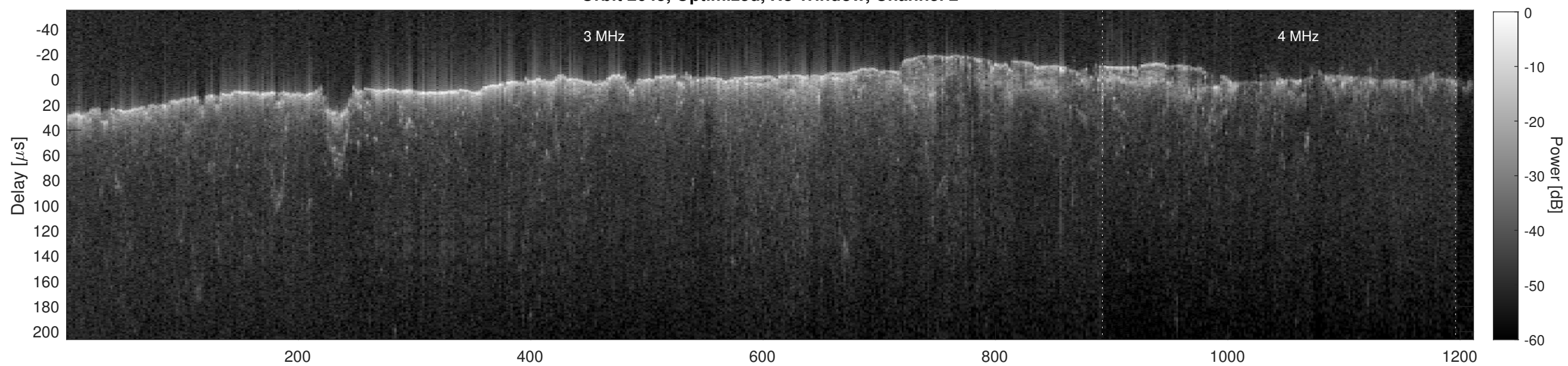
Orbit 2645, Cluttergram
