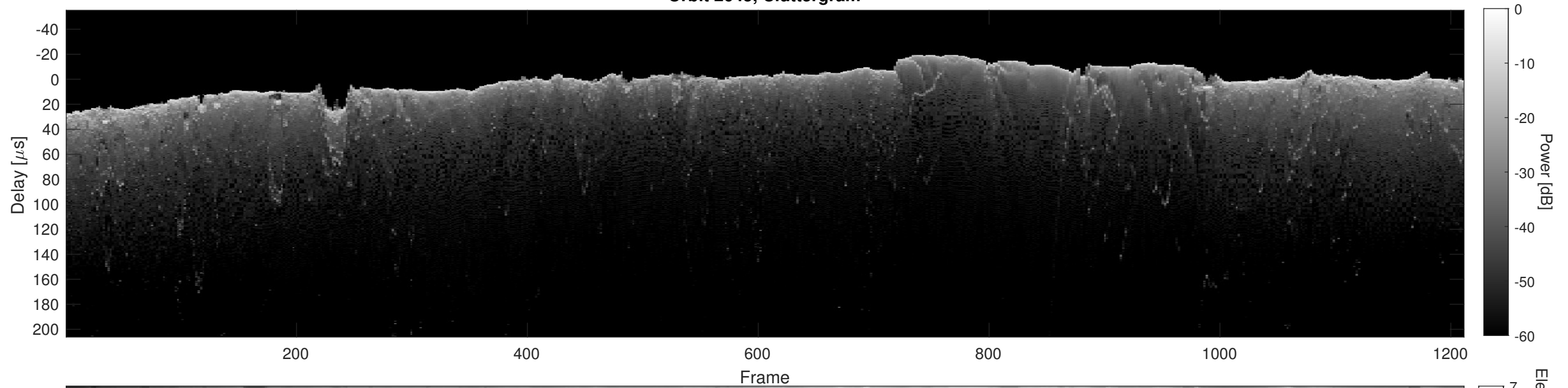
Orbit 2645, Cluttergram
