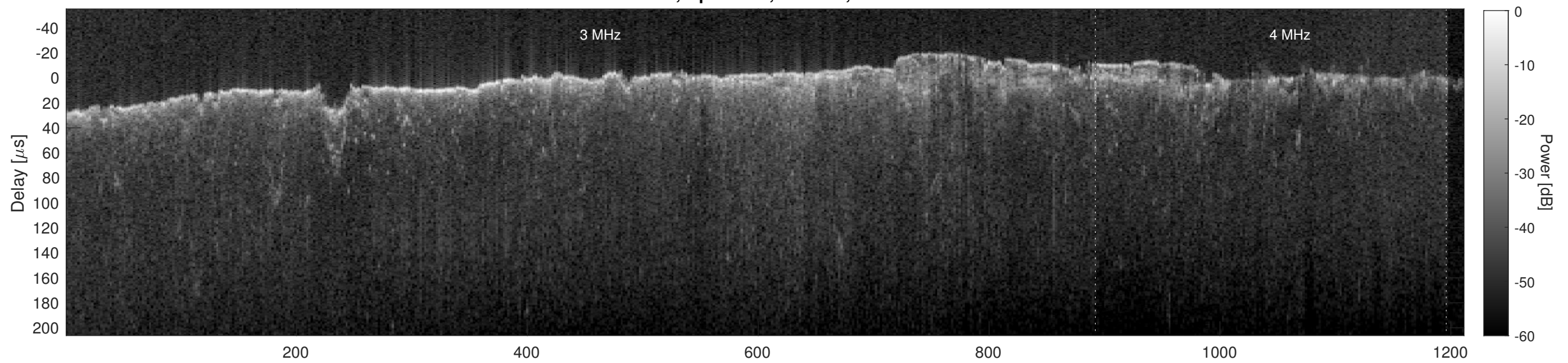
Orbit 2645, Cluttergram
