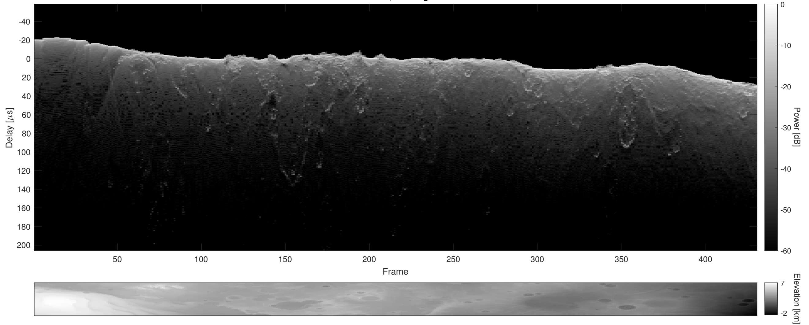
Orbit 2646, Cluttergram
