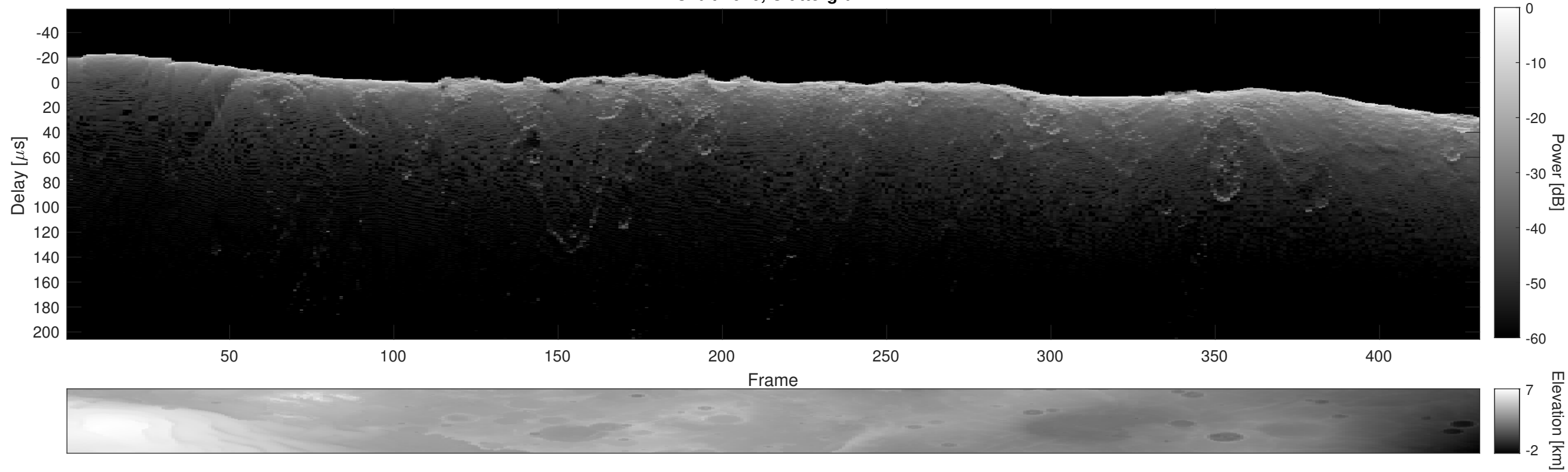
Orbit 2646, Cluttergram
