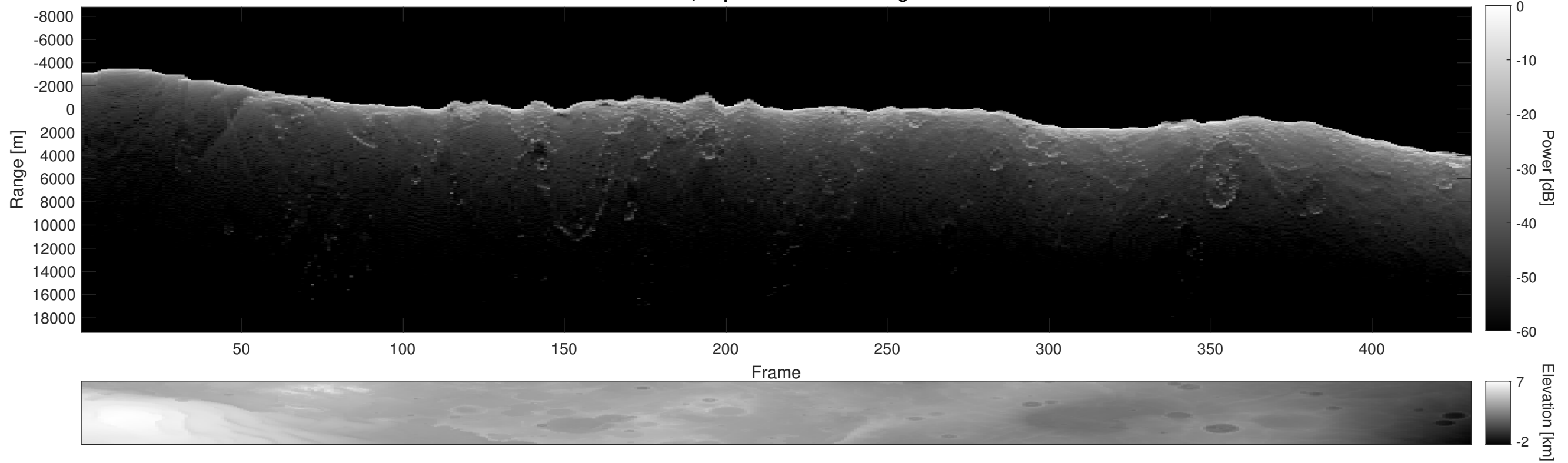
Orbit 2646, Depth-Corrected Cluttergram
