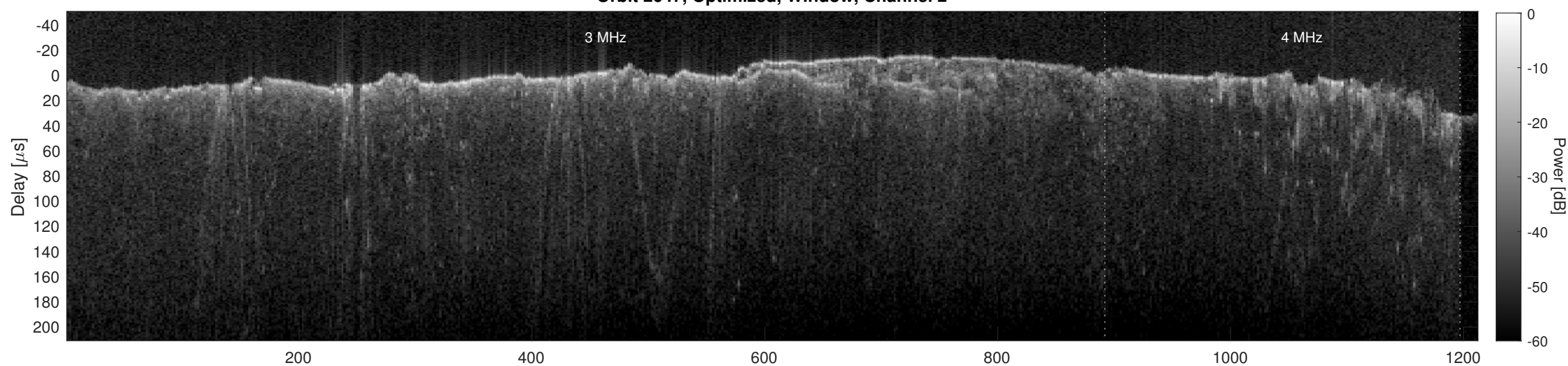
Orbit 2647, Cluttergram
