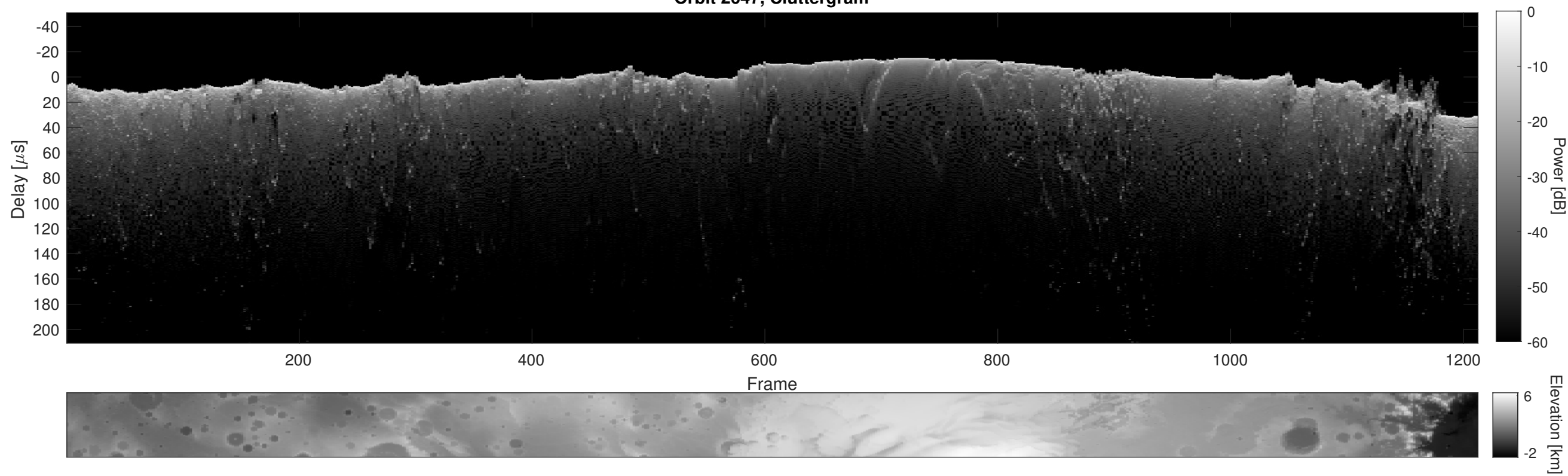
Orbit 2647, Cluttergram
