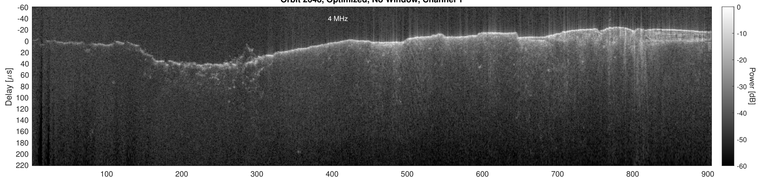
Orbit 2648, Optimized, No Window, Channel 2
