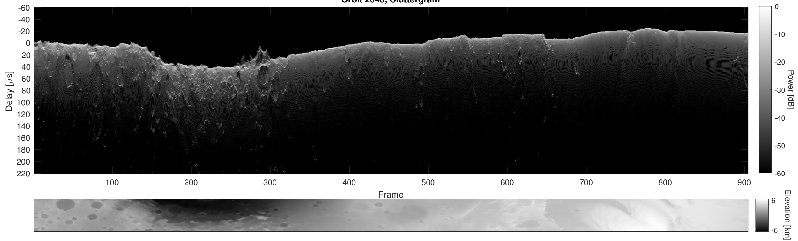
Orbit 2648, Cluttergram
