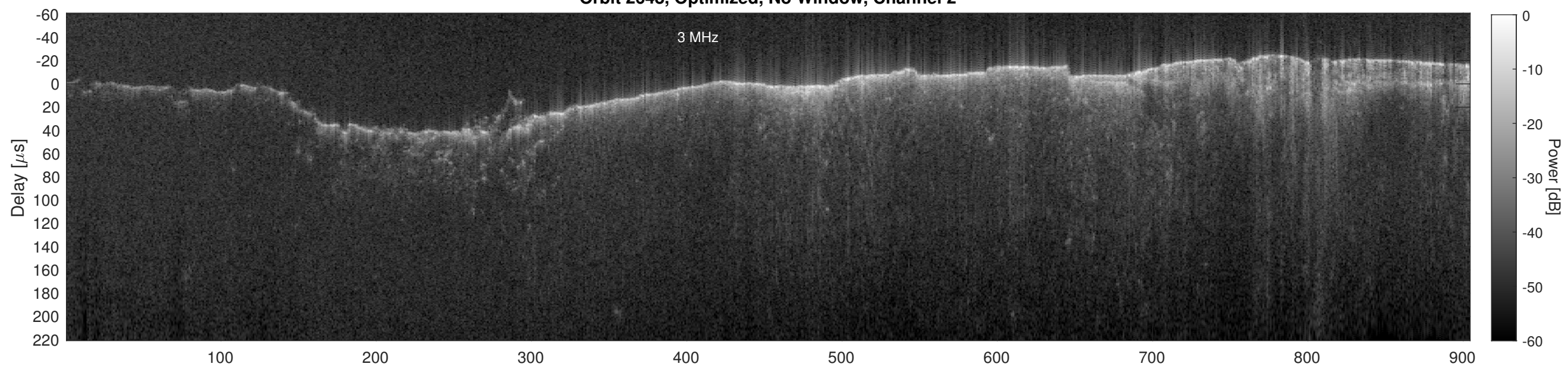
Orbit 2648, Cluttergram
