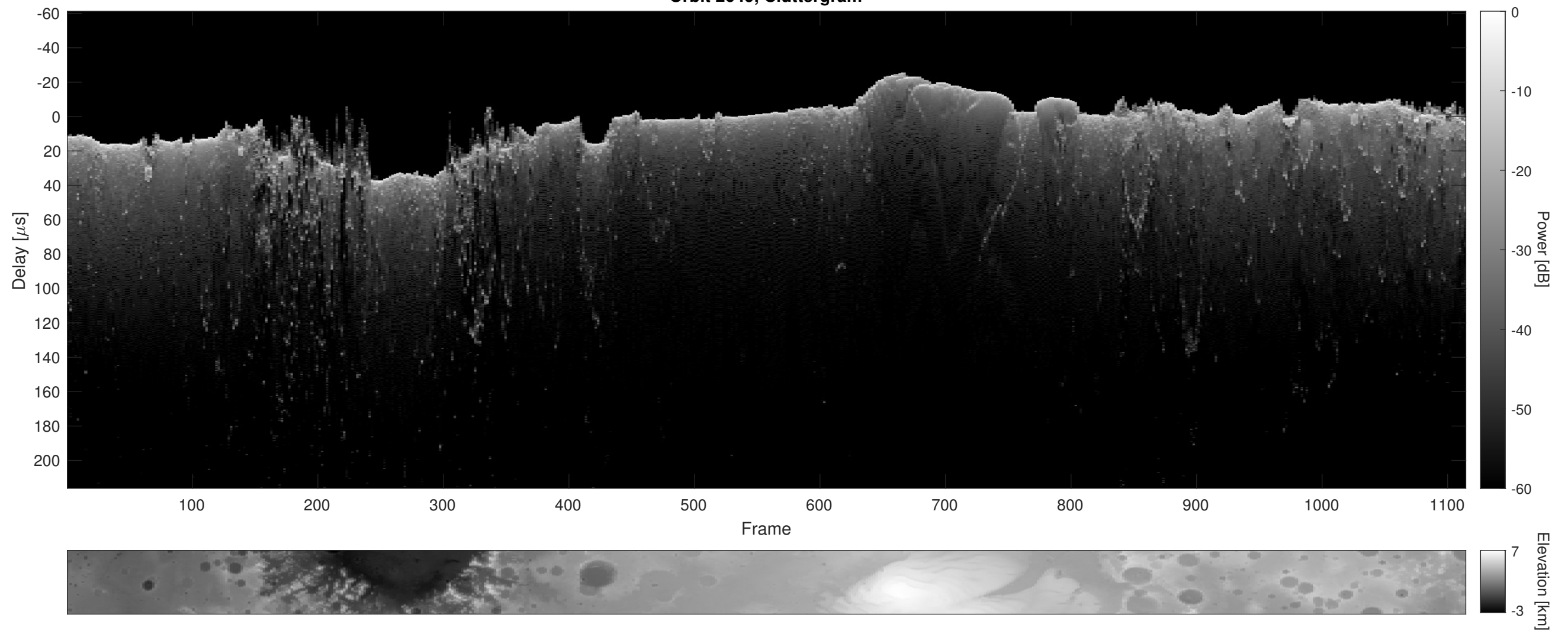
Orbit 2649, Cluttergram
