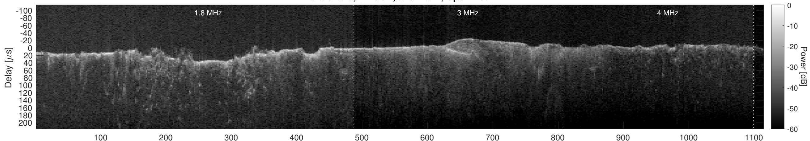
Orbit 2649, Cluttergram
