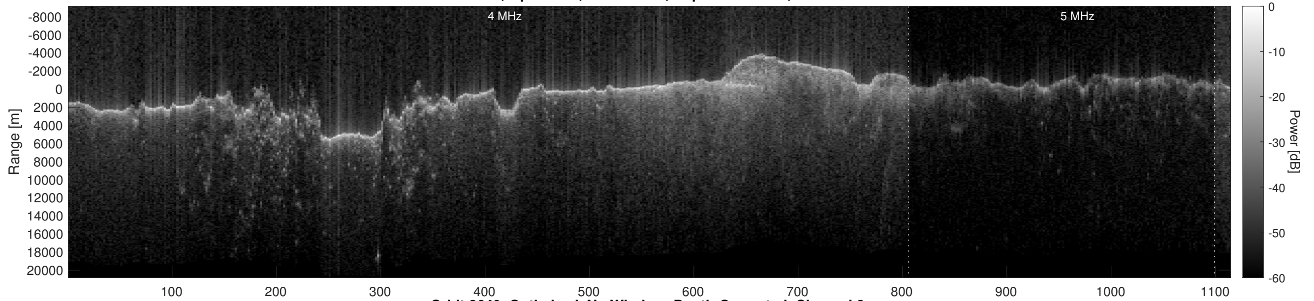
Orbit 2649, Optimized, No Window, Depth-Corrected, Channel 2
