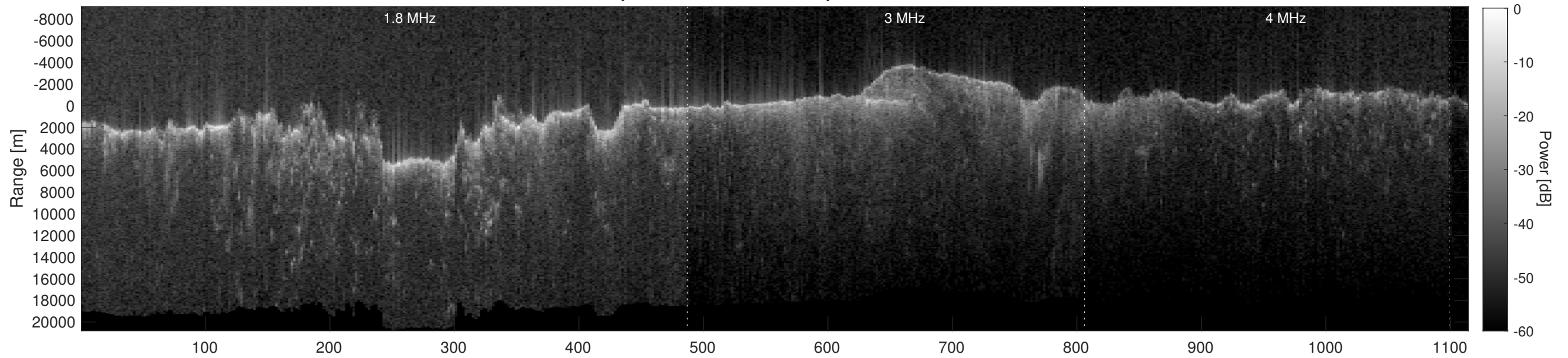
Orbit 2649, Depth-Corrected Cluttergram
