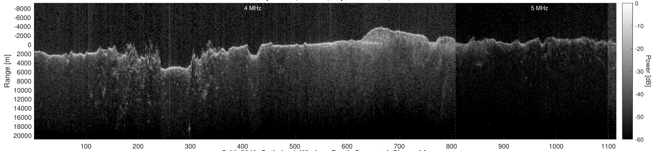
Orbit 2649, Optimized, Window, Depth-Corrected, Channel 2
