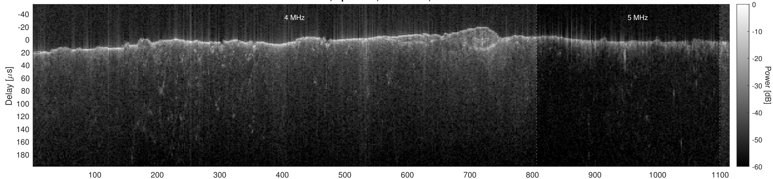
Orbit 2650, Optimized, No Window, Channel 2
