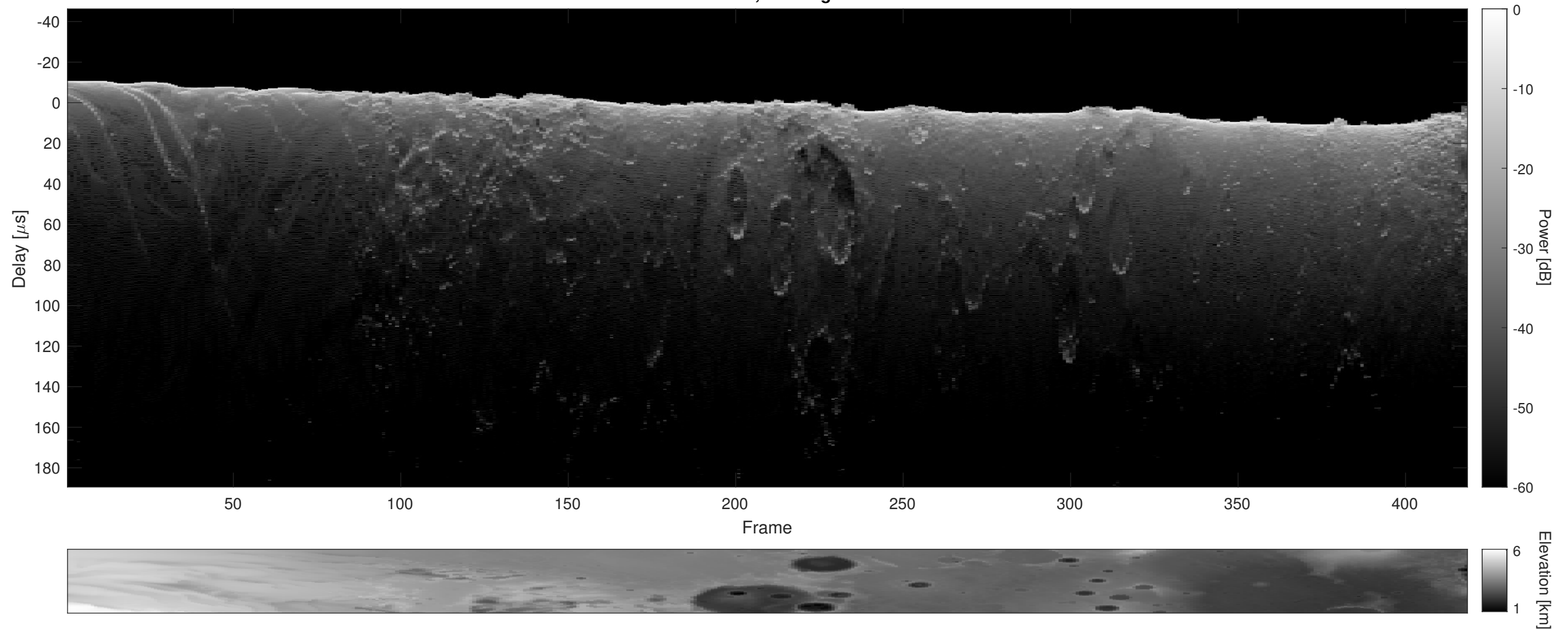
Orbit 2651, Cluttergram
