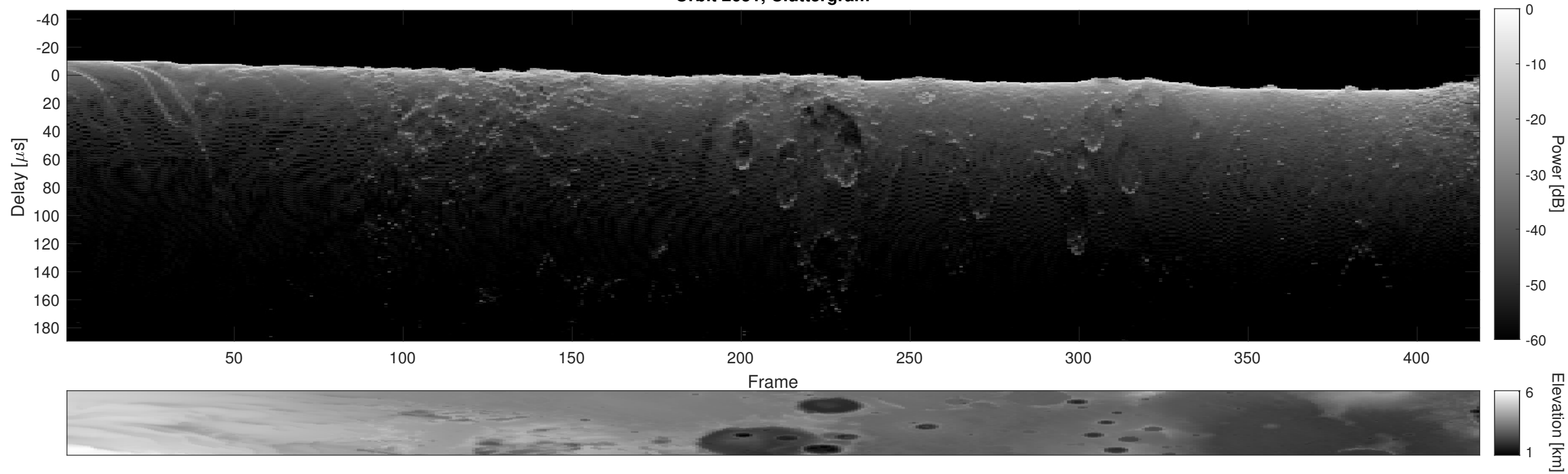
Orbit 2651, Cluttergram
