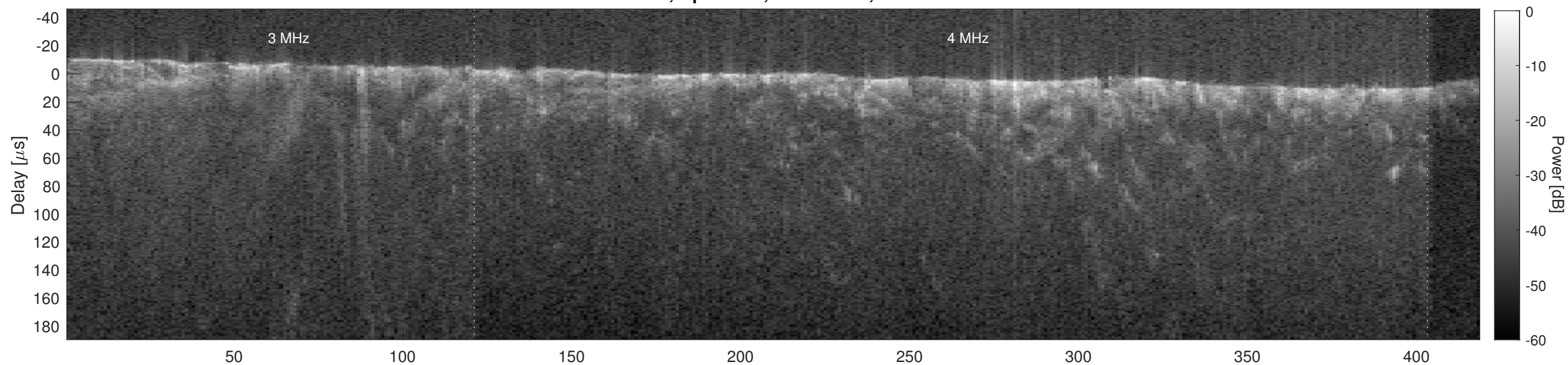
Orbit 2651, Cluttergram
