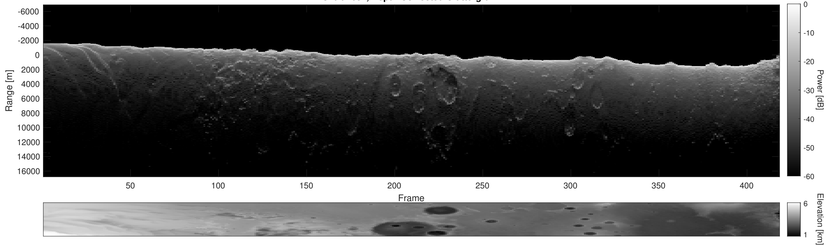
Orbit 2651, Depth-Corrected Cluttergram
