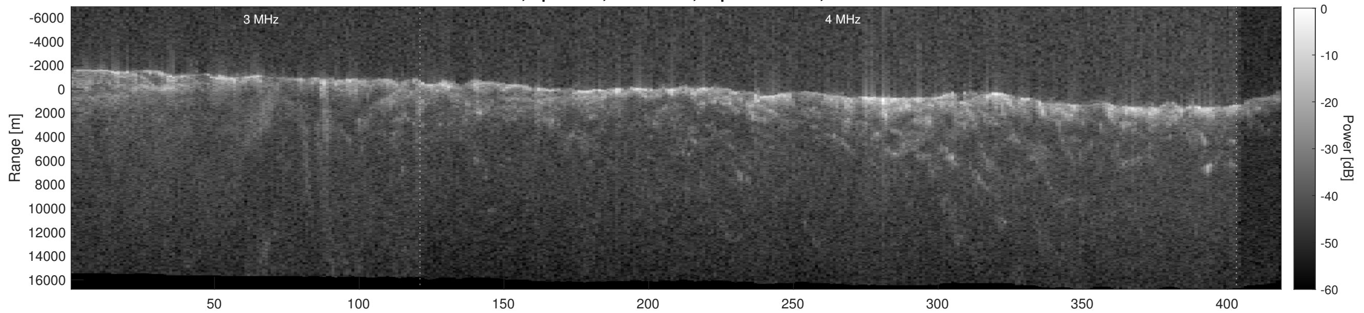
Orbit 2651, Depth-Corrected Cluttergram
