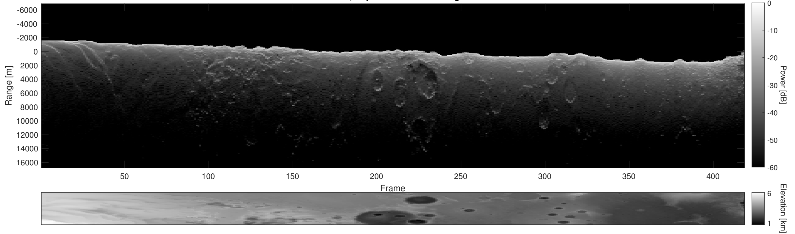
Orbit 2651, Depth-Corrected Cluttergram
