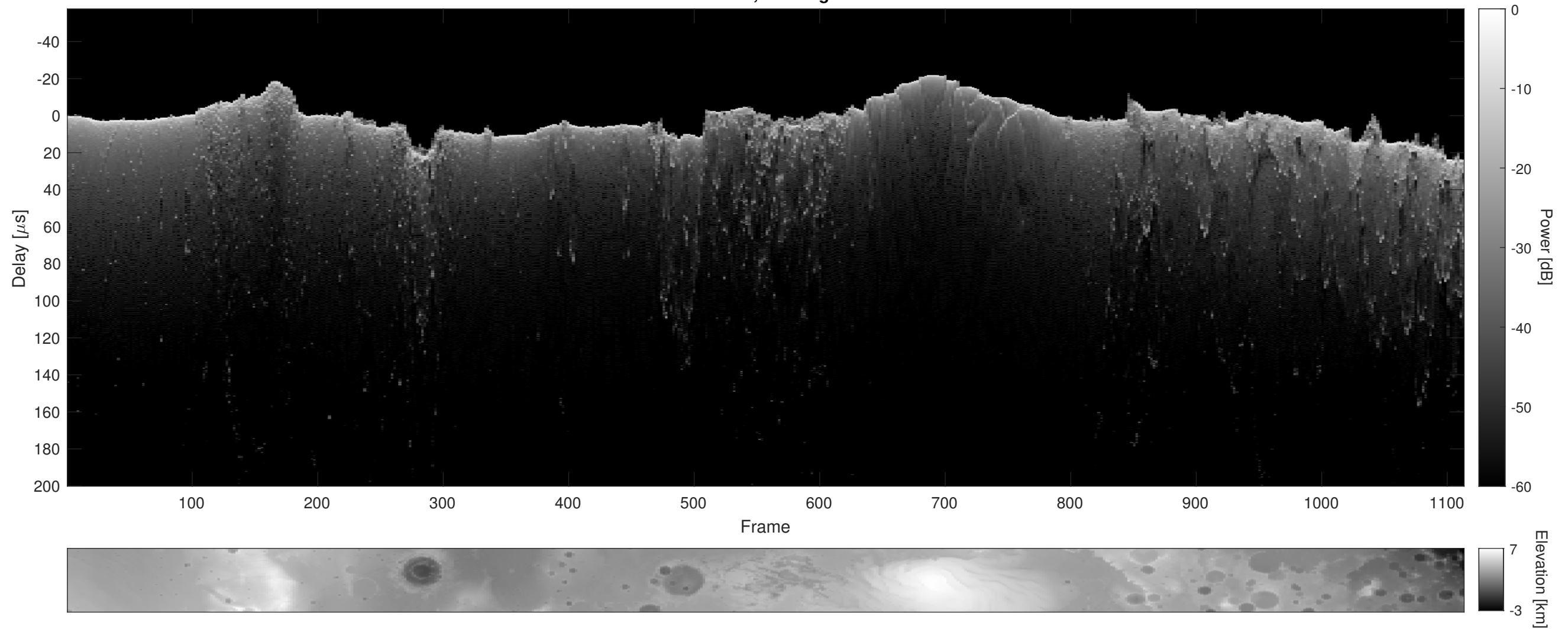
Orbit 2653, Cluttergram
