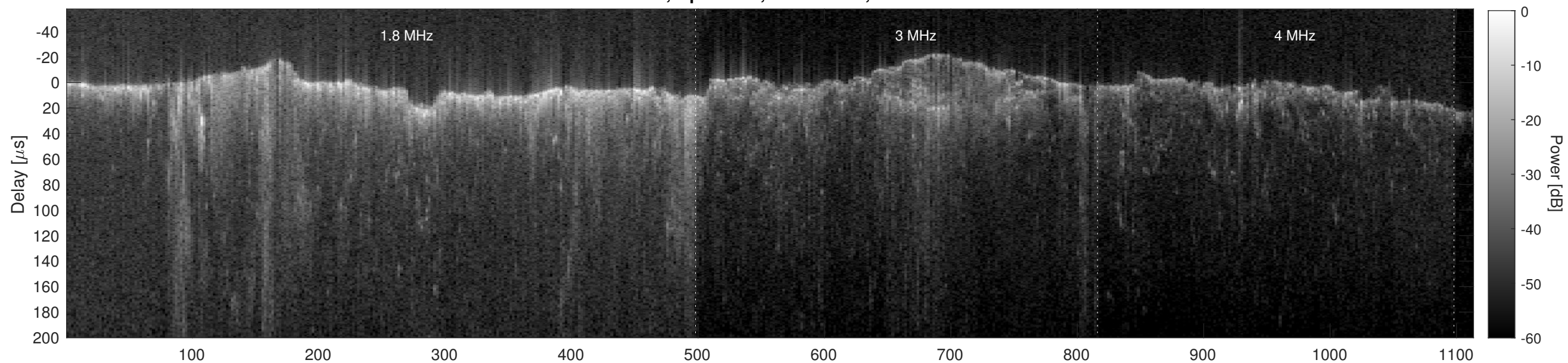
Orbit 2653, Cluttergram
