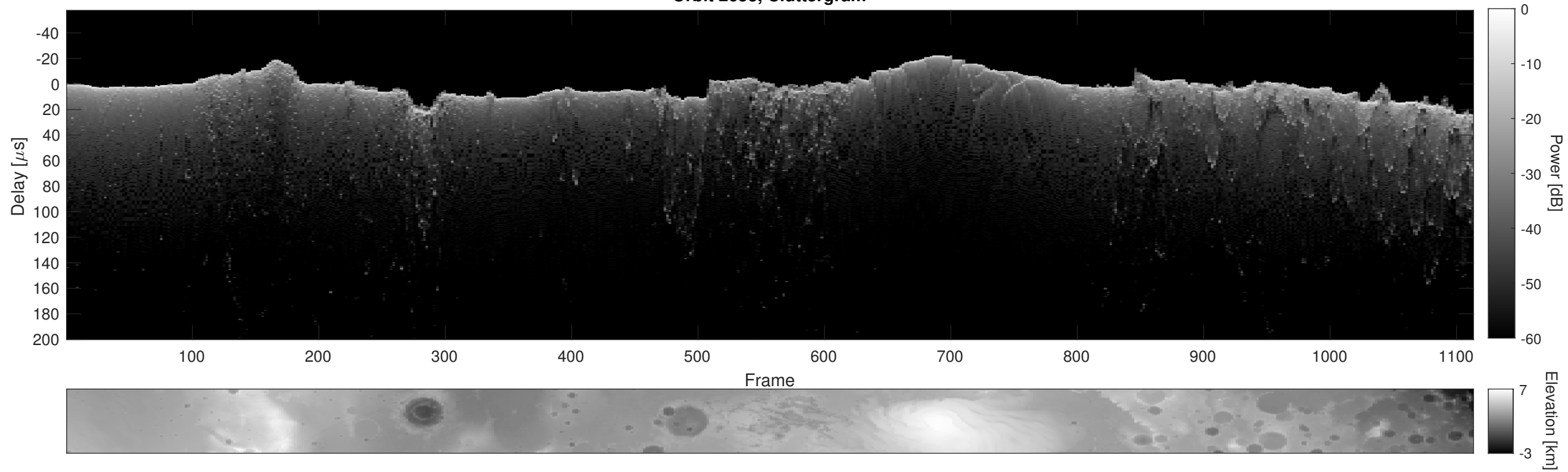
Orbit 2653, Cluttergram
