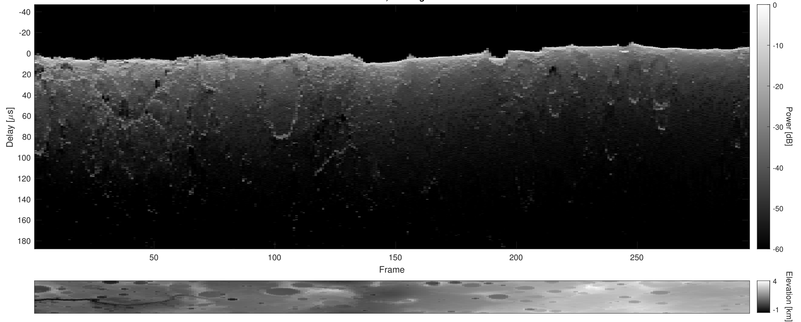
Orbit 2654, Cluttergram
