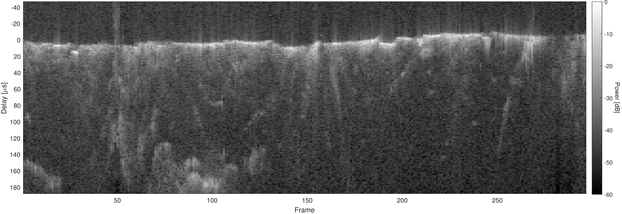
Orbit 2654, Optimized, No Window, Channel 2
